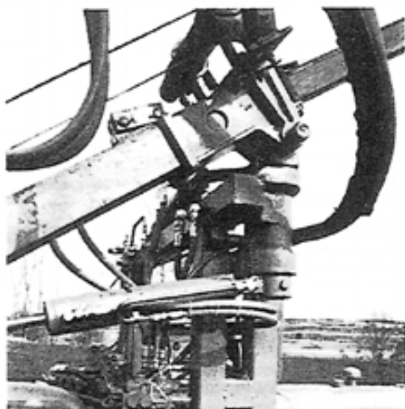
Fig. 4. The tough outer cover of a hose assembly will abrade if exposed to continuous rubbing in the same spot. To avoid this problem, route and clamp to keep hose clear from interfering objects.
