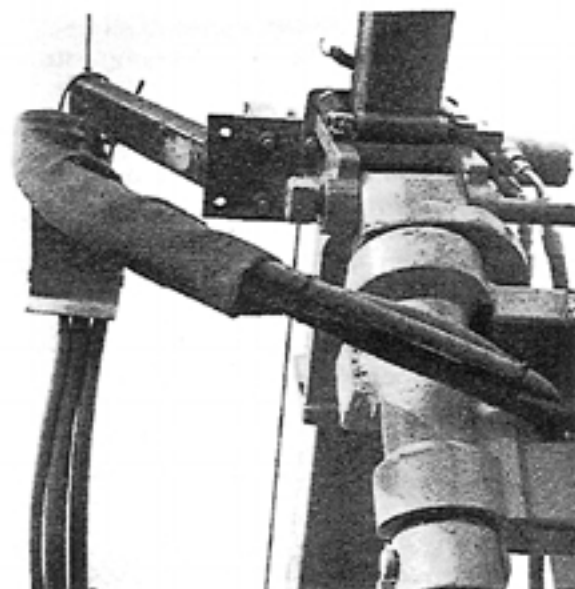
Fig. 5. The choice of sheathing and clamping bundles of hose assemblies must be studied carefully. Hose should be routed to provide proper clamping, yet allow for flexing when pressurized.
