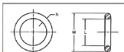
Basic O-Ring dimensions are shown for reference only
