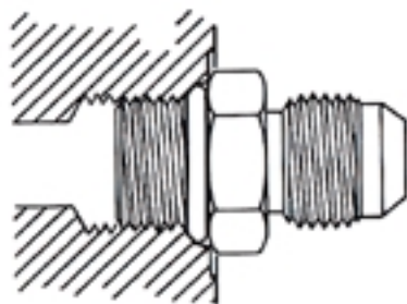
SAE O-Ring boss connection
