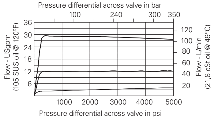
TYPICAL FLOW REGULATION
