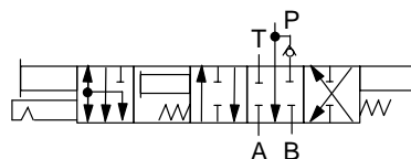
“C” Spool (CM2 only)
